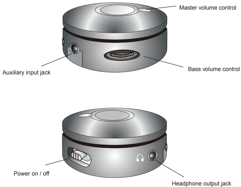
Multi-function Control Pod
